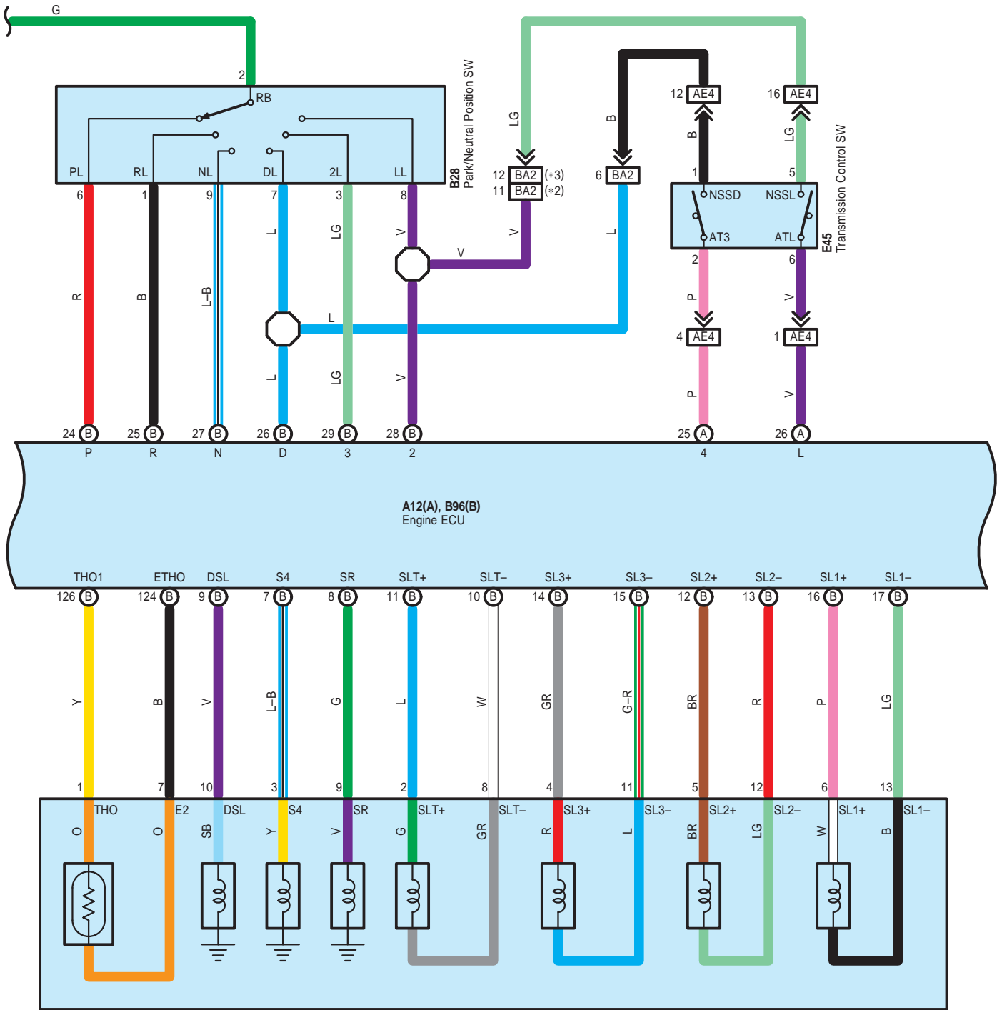
B66 ECT Solenoid
