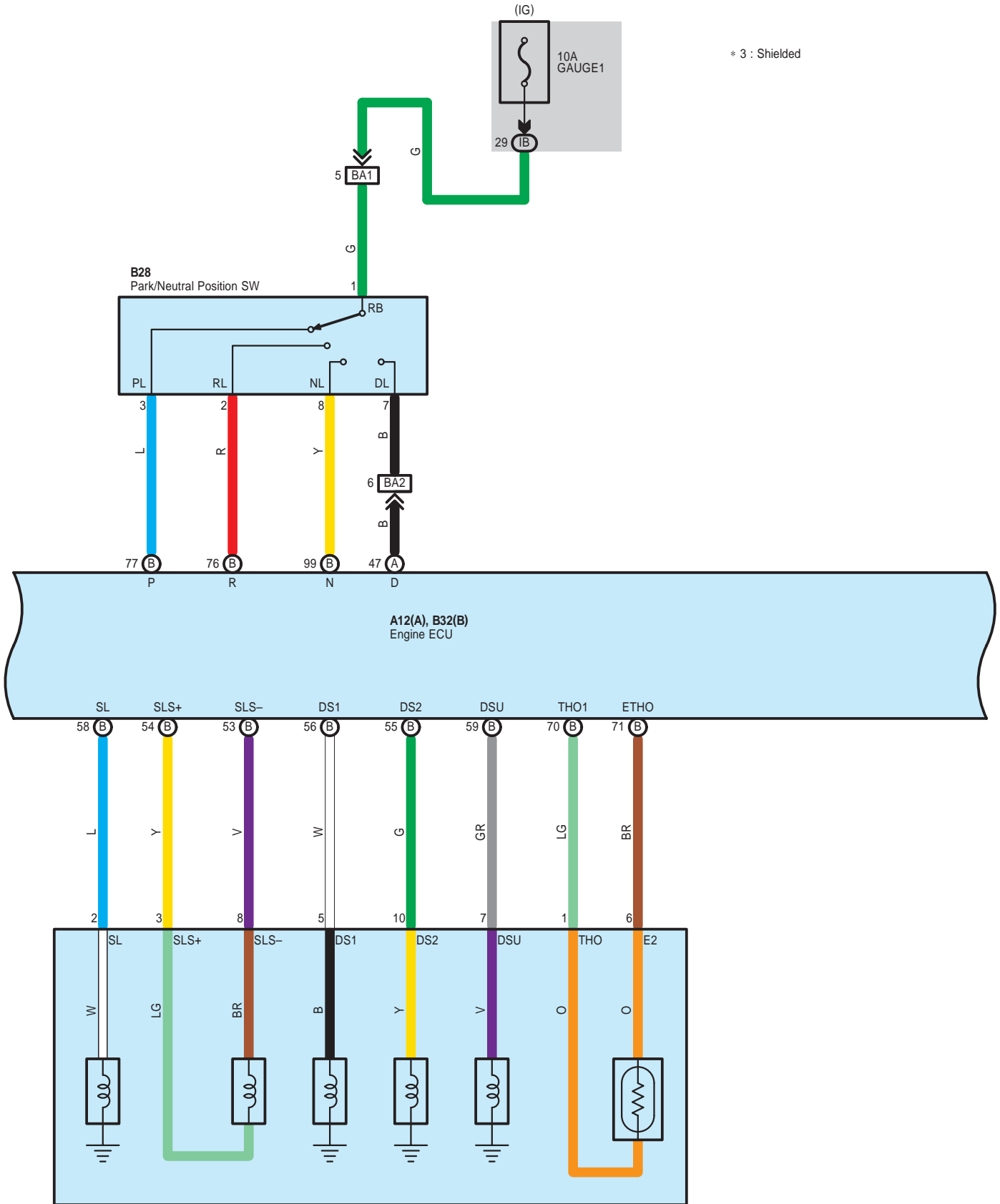
B29 ECT Solenoid
