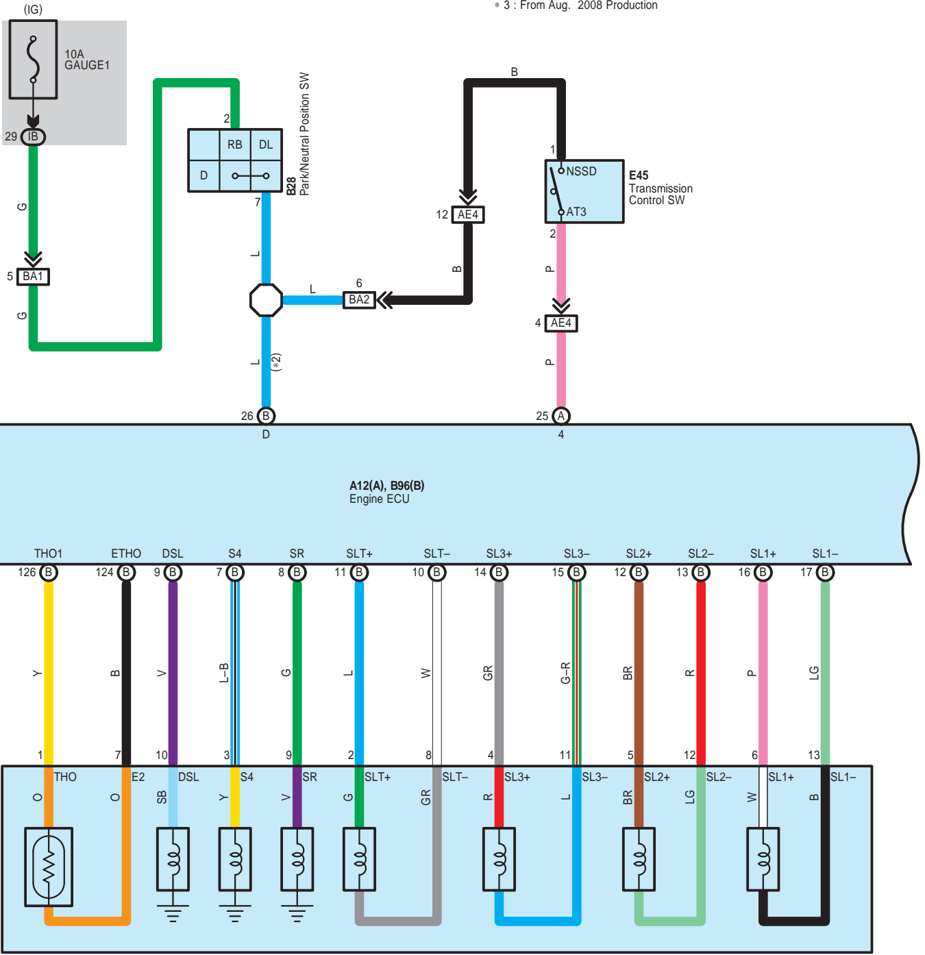
B66 ECT Solenoid
