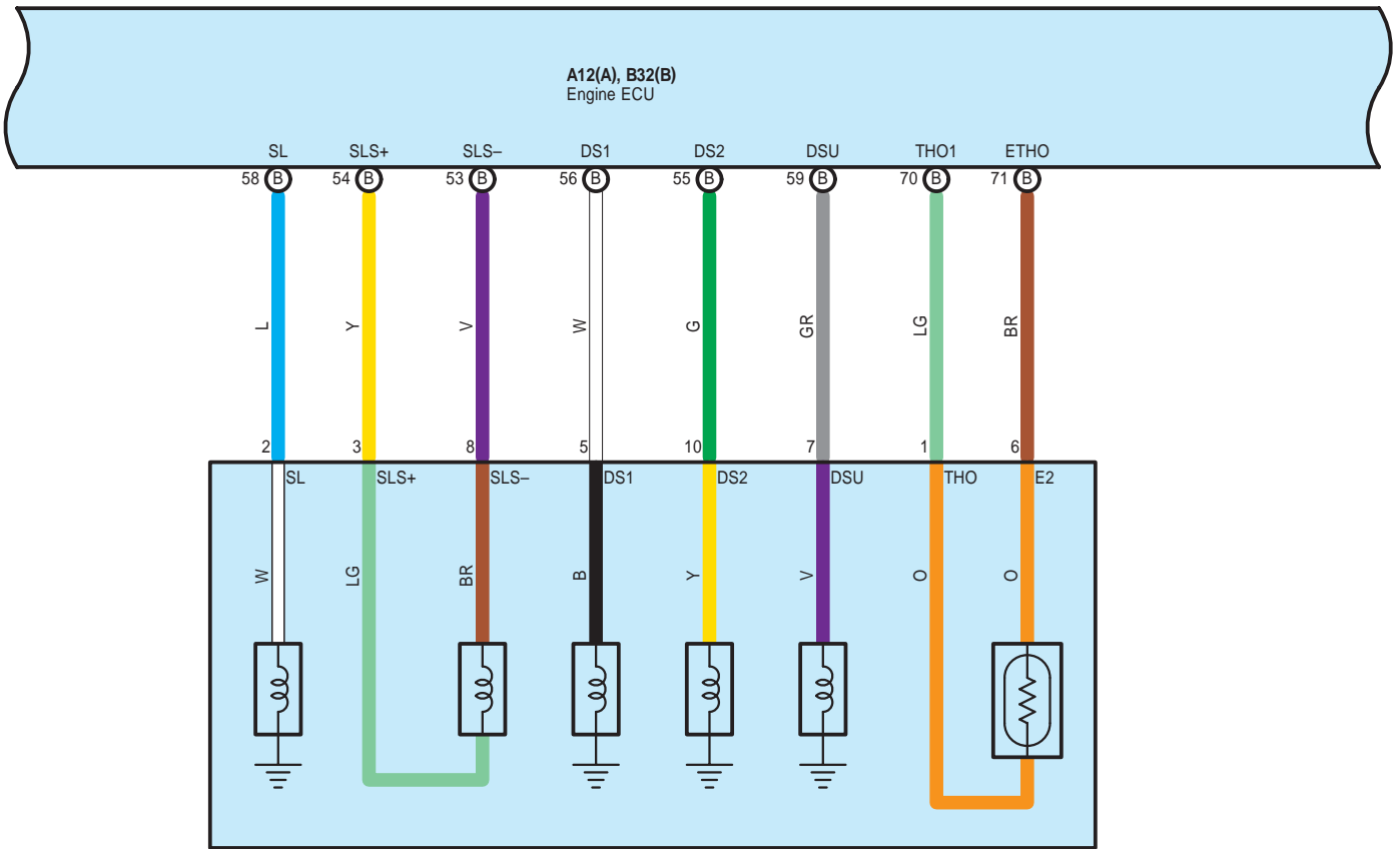
B29 ECT Solenoid
