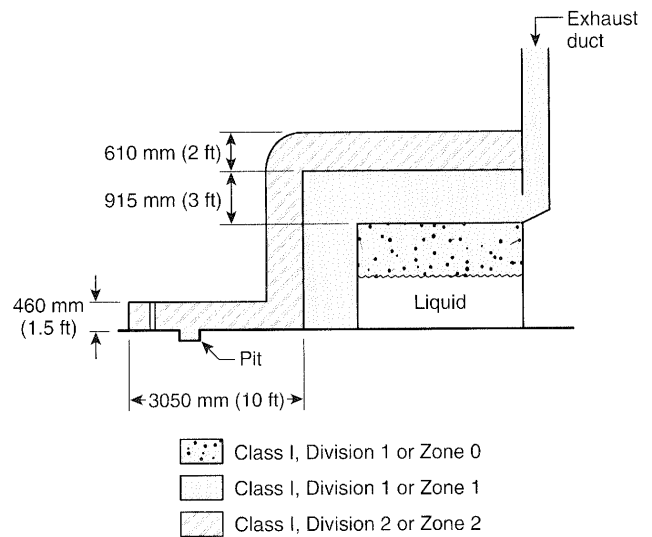
Figure 516.3(D)(6)(c) Electrical Area Classification for Open Dipping and Coating Processes with Partial Peripheral Vapor Containment and Ventilation — Vapors NOT Confined to Process Equipment. [34:Figure 6.4(c)]
