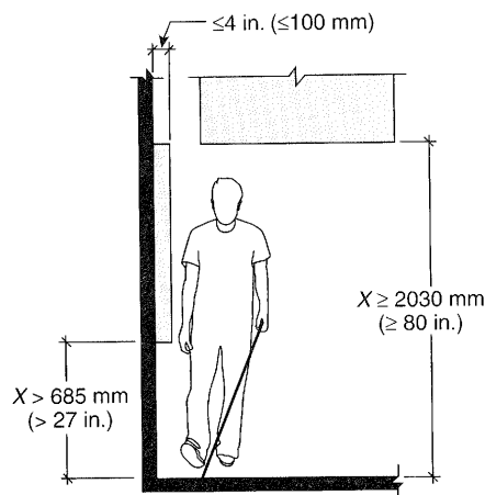
Figure J.2 Limits of Protruding Objects.
