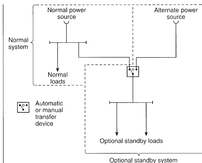
Figure 702.2 Optional Standby Systems.
