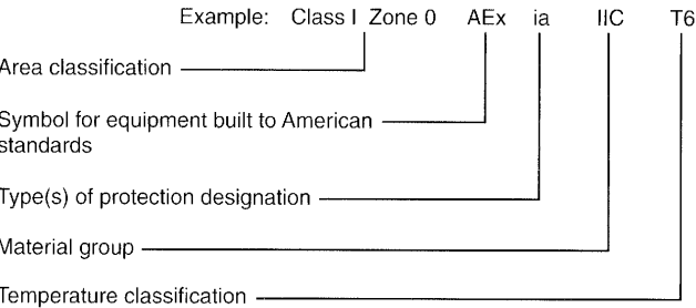
Informational Note Figure 505.9(C)(2), No. 1, Zone Equipment Marking.
