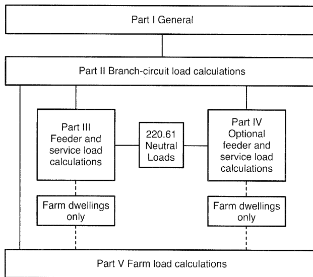
Figure 220.1 Branch-Circuit, Feeder, and Service Load Calculation Methods.
