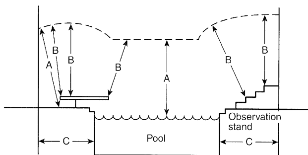
Figure 680.8(A) Clearances from Pool Structures.
