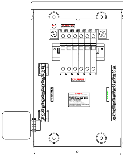
MNPV6 shown with breakers & lightning arrestor
