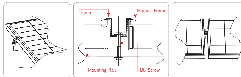
Module installed using Clamp Fitting method
