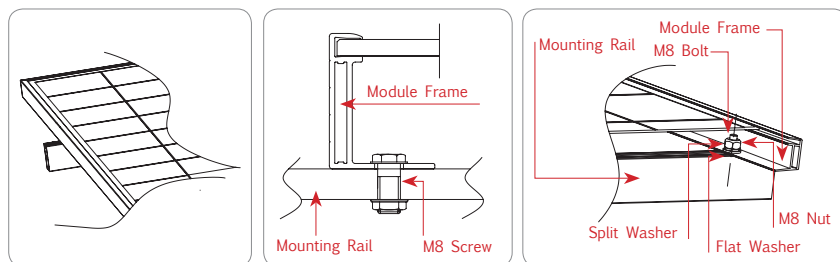
Module installed using Screw Fitting method
