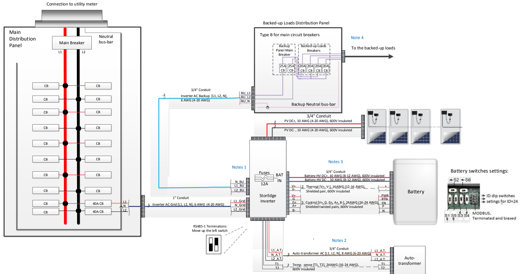
Figure 36: Backup Power Only - Basic Configuration
