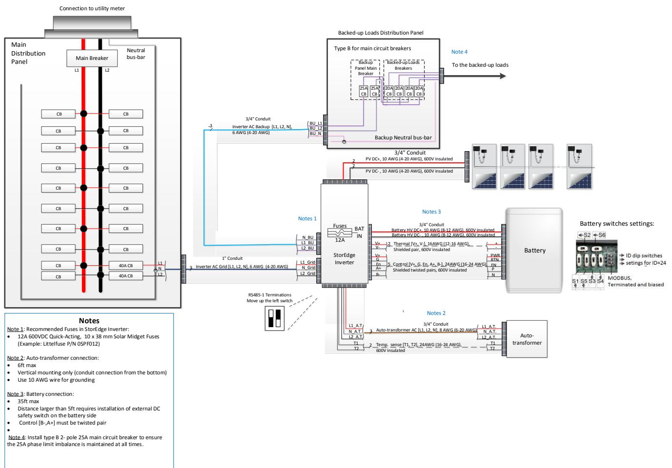
Figure 14: Backup Power only - Basic Configuration
