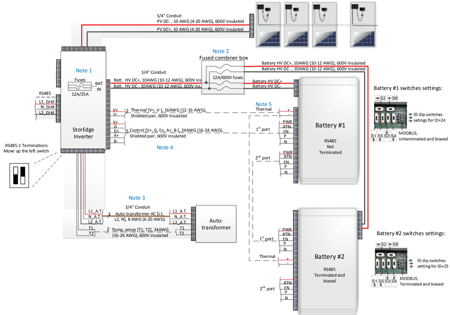
Figure 34: Backup Power with Smart Energy Management - Two-Battery Configuration, Batteries – StorEdge Inverter Connection
