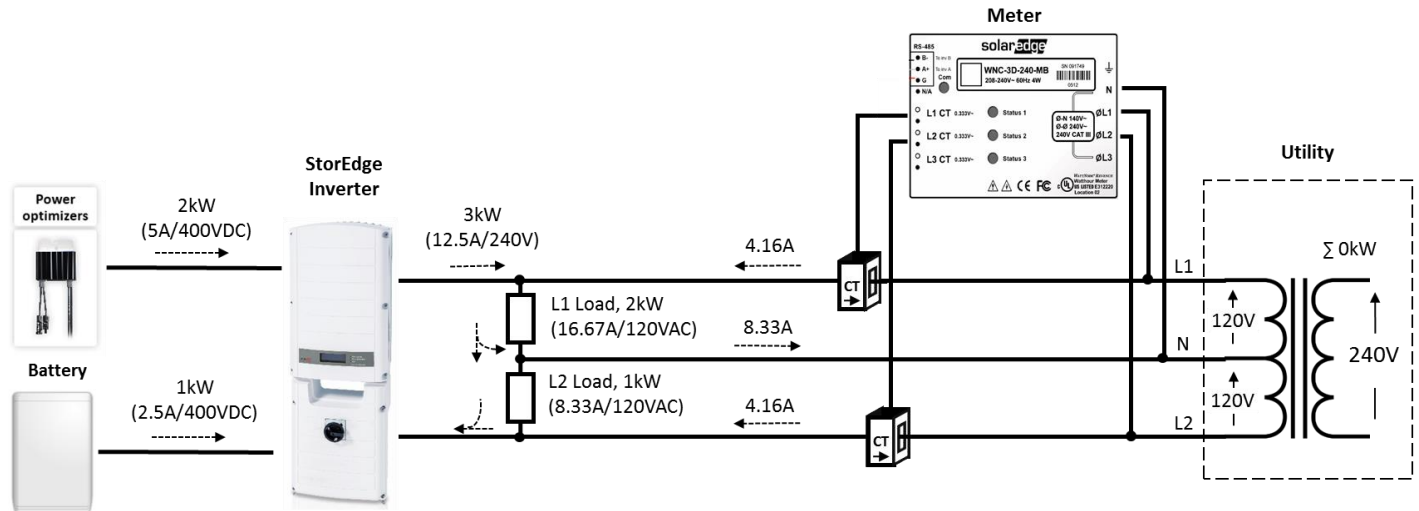
Figure 29: Power Production Flow
