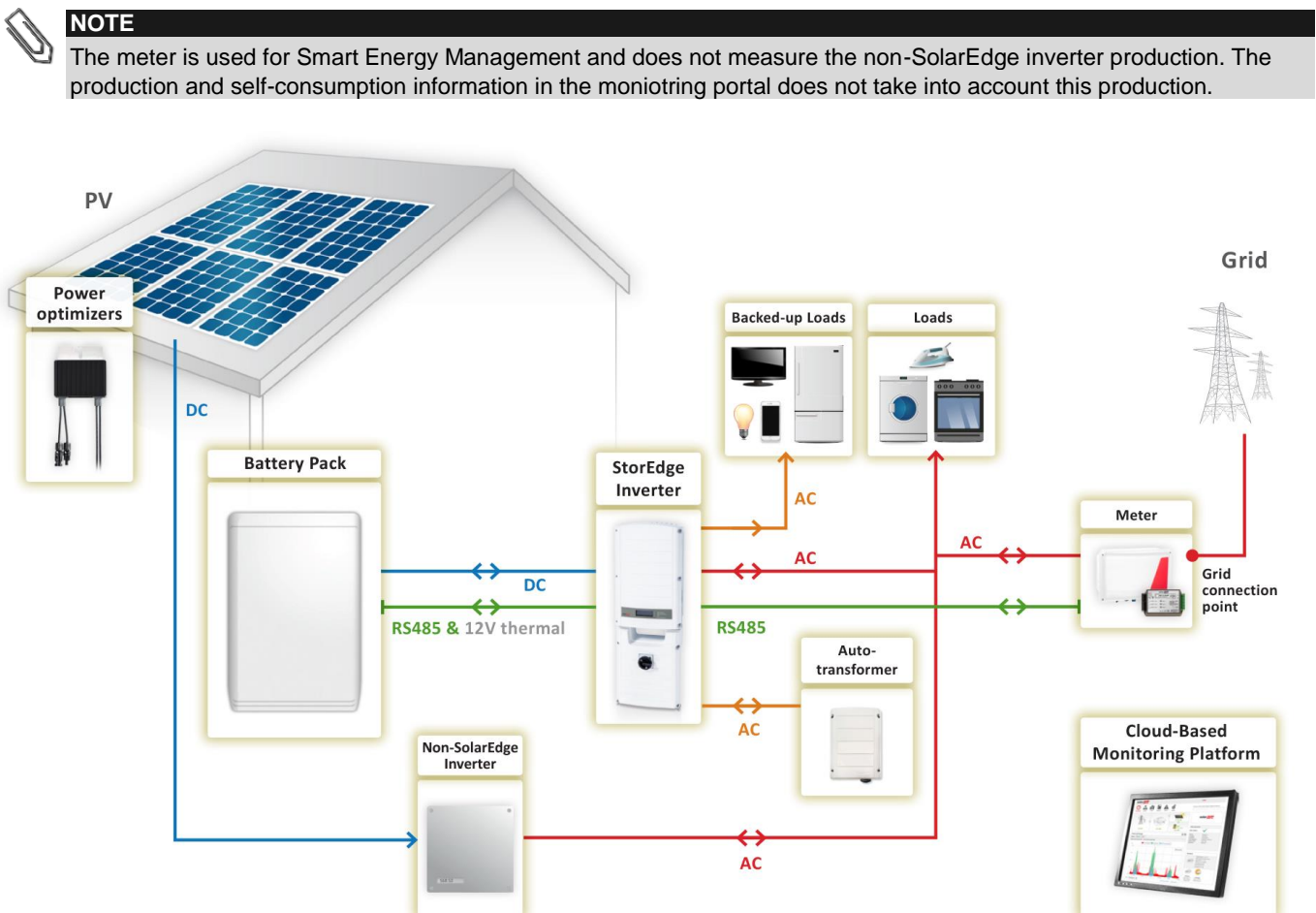
Figure 12: Backup Power with Smart Energy Management - AC Coupling using a non-SolarEdge Inverter
