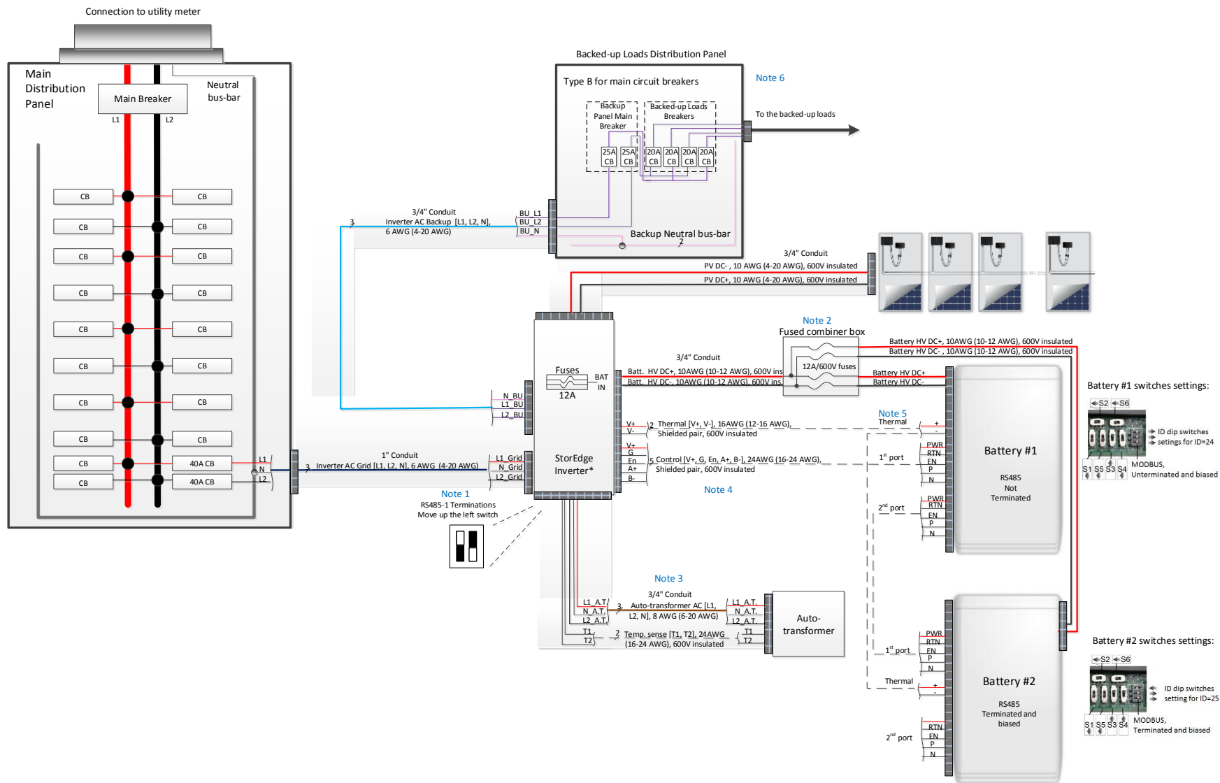
Figure 39: Backup Power Only – Two Battery Configuration
