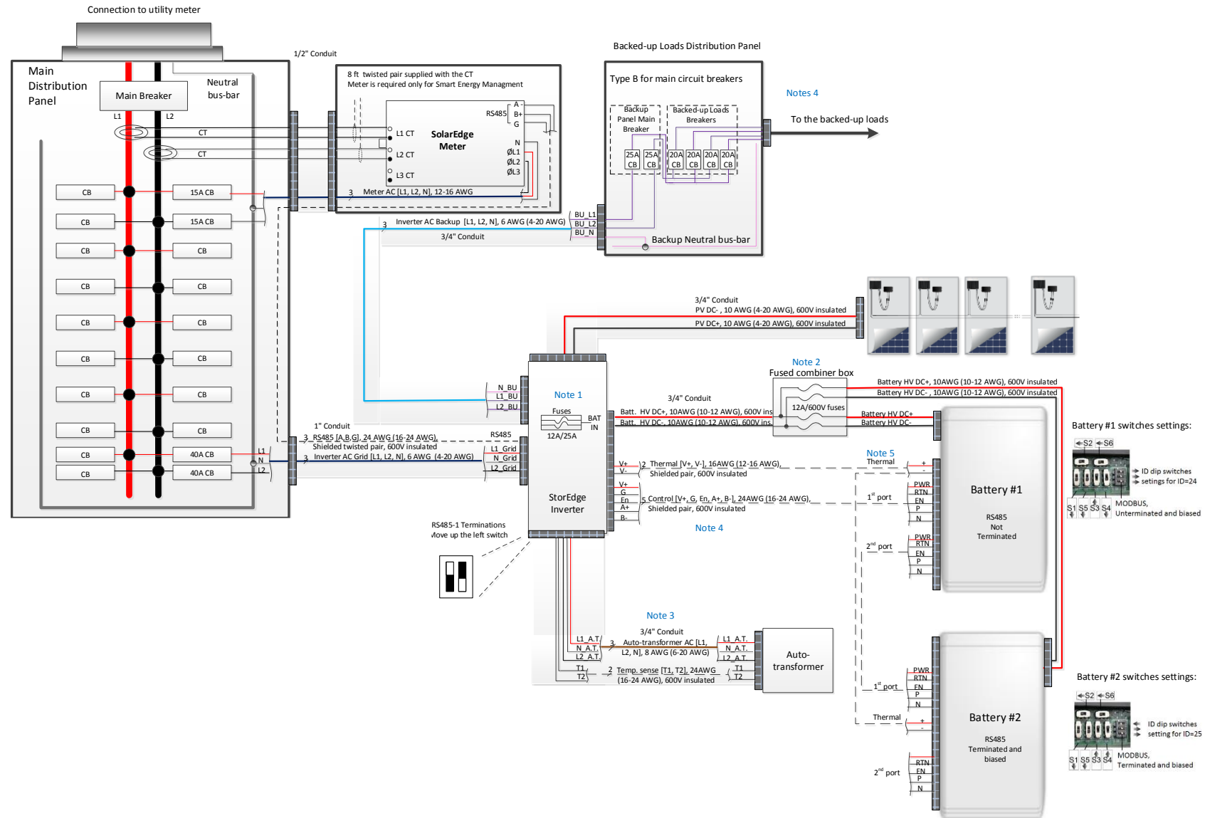
Figure 33: Backup Power with Smart Energy Management - Two-Battery Configuration
